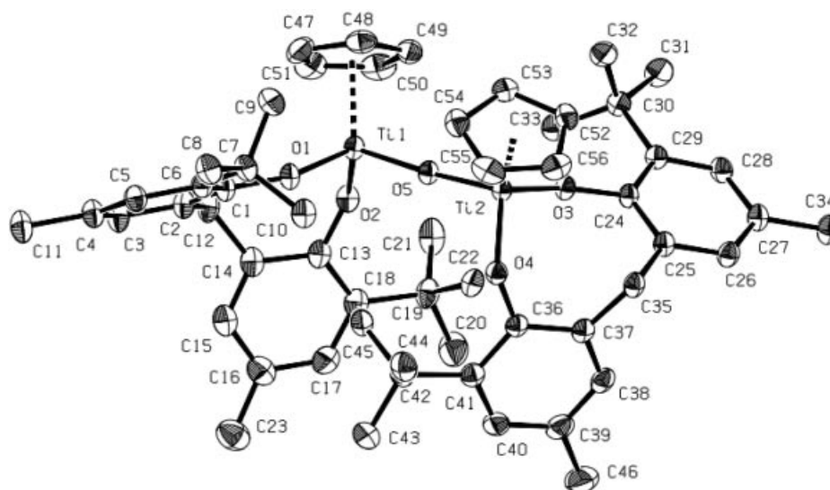
Figure 4. ORTEP plot of compound 11 in the solid state. Thermal ellipsoids are drawn at the 40% probability level. Hydrogen atoms are omitted for clarity.
