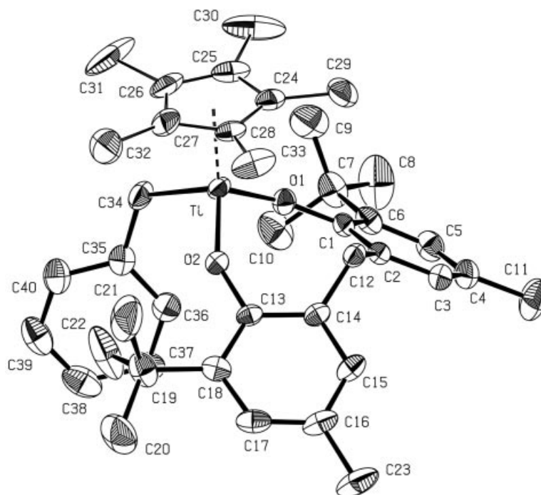
Figure 2. ORTEP plot of compound 8 in the solid state. Thermal ellipsoids are drawn at the 50% probability level. Hydrogen atoms are omitted for clarity.
