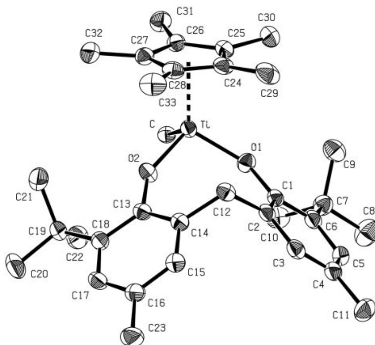
Figure 3. ORTEP plot of compound 9 in the solid state. The major part (82.1%) of the disordered Cp ligand is shown. Thermal ellipsoids are drawn at the 50% probability level. Hydrogen atoms are omitted for clarity.
