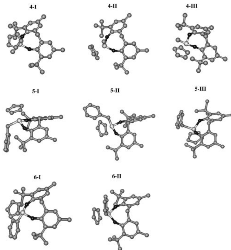
Figure 1. Optimised structures for [\text{TiR}'\text{Cp}(\eta^2\text{-mbmp})] [ \text{R}' = \text{Me} ( 4 ), \text{CH}_2\text{Ph} ( 5 ), \text{Ph} ( 6 )] complexes.
